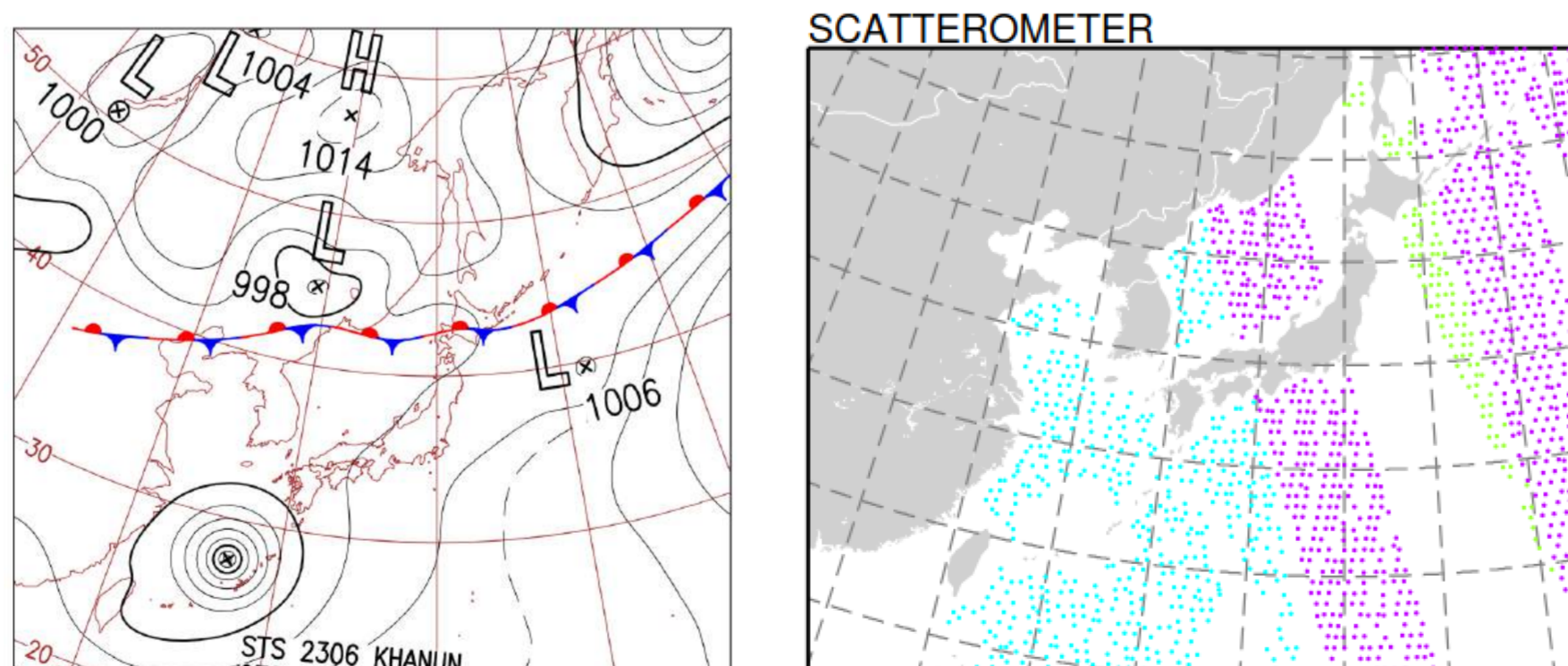
Fig.7 Data distribution of assimilated scatterometer data between 09 - 12 UTC 5 Aug. 2023
