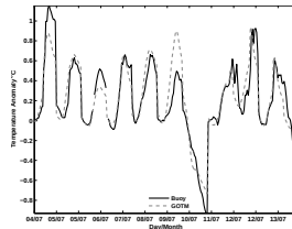
Figure: Diurnal variability at 2 m depth from July 4th to 14th, 2013.
