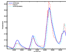
Figure: Modelled SST with different forcing.
