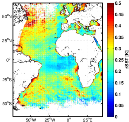
Figure: Maximum mean monthly warming, SST_{day} - SST_{found} .
