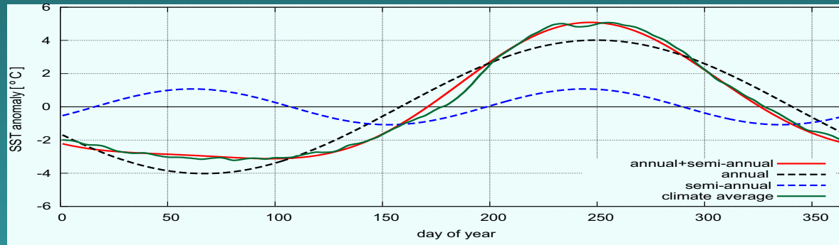
Figure 1 Time variation of SST at 45°N, 145°W.
