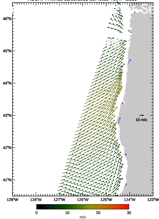
ASCAT A winds 02/09/2015 18:46:25 rev # 43119
