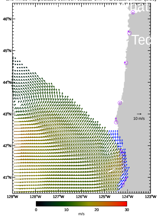
X1 Rapidscat V1.1 winds 02/09/2015 08:39:12 rev # 02157 and winds interpolated between coastal CMAN & scatterometer (blue)
