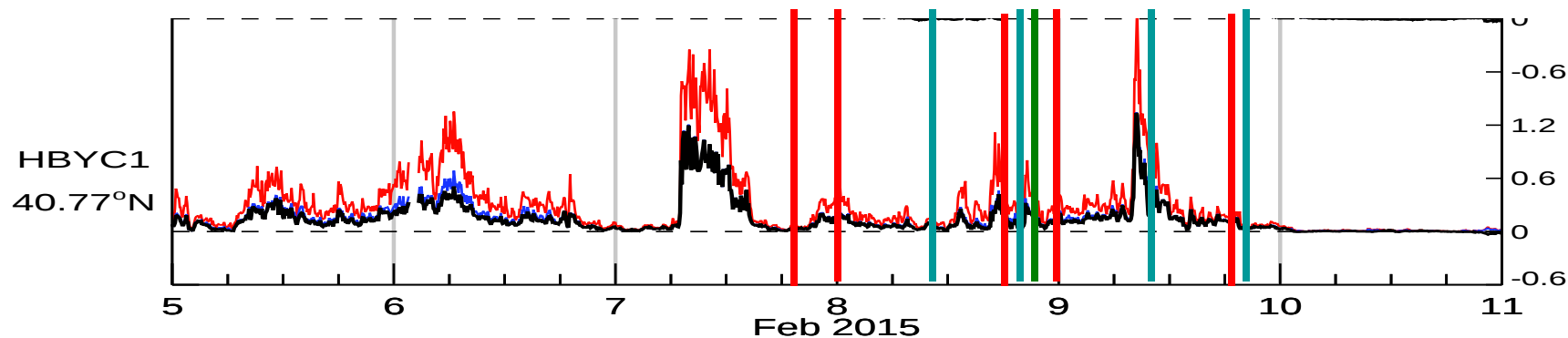
X1 Rapidscat V1.1 winds 02/09/2015 08:39:12 rev # 02157 and winds interpolated between coastal CMAN & scatterometer (blue)
