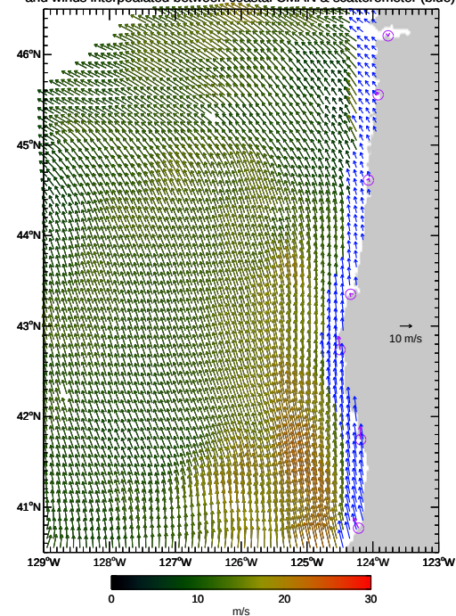
X1 Rapidscat V1.1 winds 02/09/2015 02:28:55 rev # 02153 and winds interpolated between coastal CMAN & scatterometer (blue)
