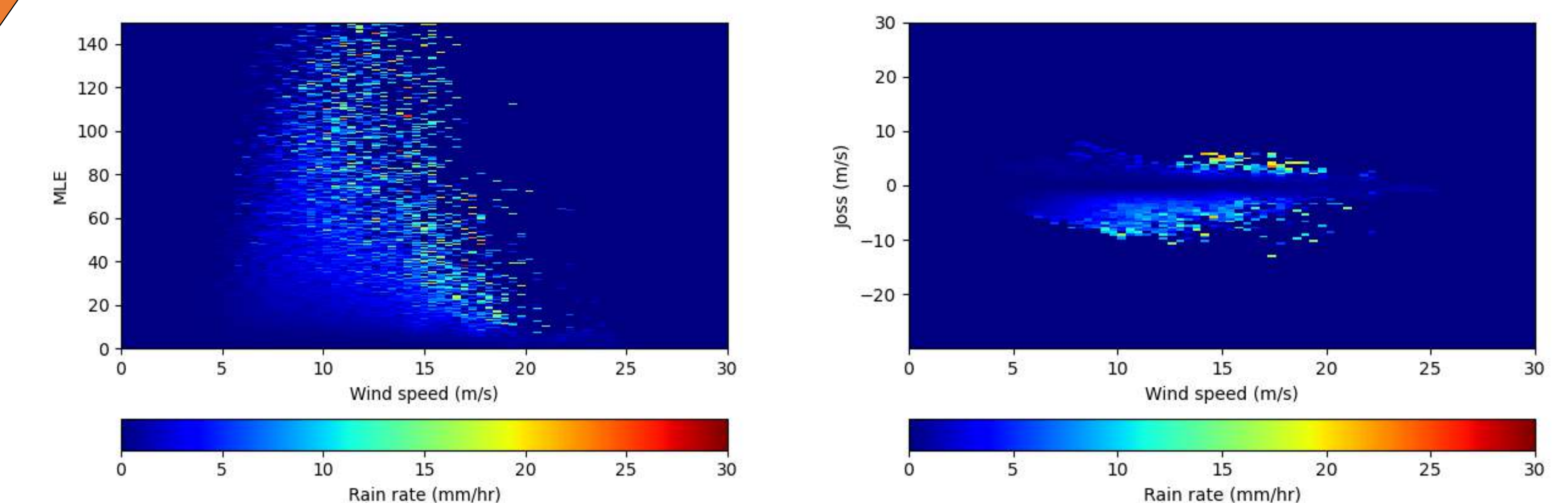
Figure 4. All the winds (Ku-band), Left: MLE collocation with rain as a function of wind speed; Right: Joss collocation with rain as a function of wind speed.
