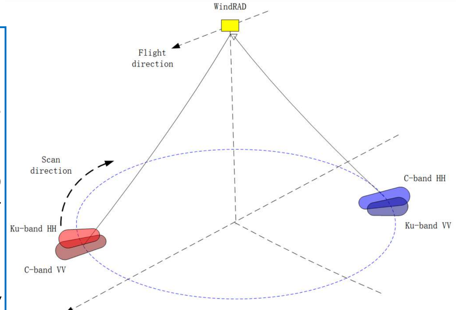
Figure 1. WindRAD scatterometer illustration plot.
